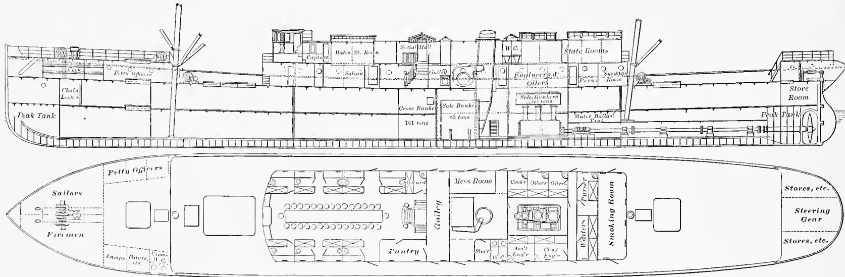
THE RED D LINE STEAMSHIP CURACOA.—Built by Wm. Cramp &amp; Sons, Philadelphia, Pa.
